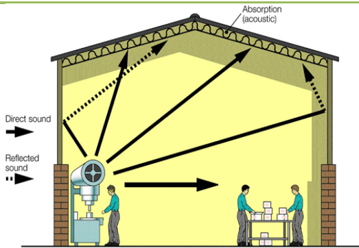
Added absorption to roof 'soaks' up reflected noise
